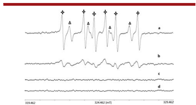
Figure 1. ESR spectra of various mixtures under irradiation of visible light for 6 min: (a) mixture of 1a (50 mM), fac -Ir(ppy) 3 (1 mol %), TBA (50 mM), 2 (50 mM), and DMPO (100 mM) in CH 3 CN; (b) mixture of 1a (50 mM), [ fac -Ir(ppy) 3 ] (1 mol %), TBA (50 mM), and DMPO (100 mM) in CH 3 CN; (c) mixture of TBA (50 mM), fac -Ir(ppy) 3 (1 mol %), 2 (50 mM), and DMPO (100 mM) in CH 3 CN; (d) mixture of 1a (50 mM), fac -Ir(ppy) 3 (1 mol %), 2 (50 mM), and DMPO (100 mM) in CH 3 CN.
