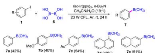
Scheme 4. Visible-Light Photoredox Borylation of 1 with 6
