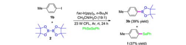
Scheme 1. Control Experiment in the Presence of PhSeSePh for Mechanism Investigation
